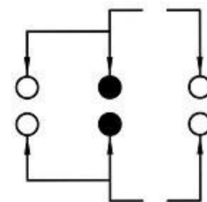
SCHEMATIC (NON-SHORTING)
